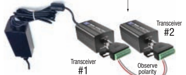
Step Two: Remove Label; Connect Hardware
