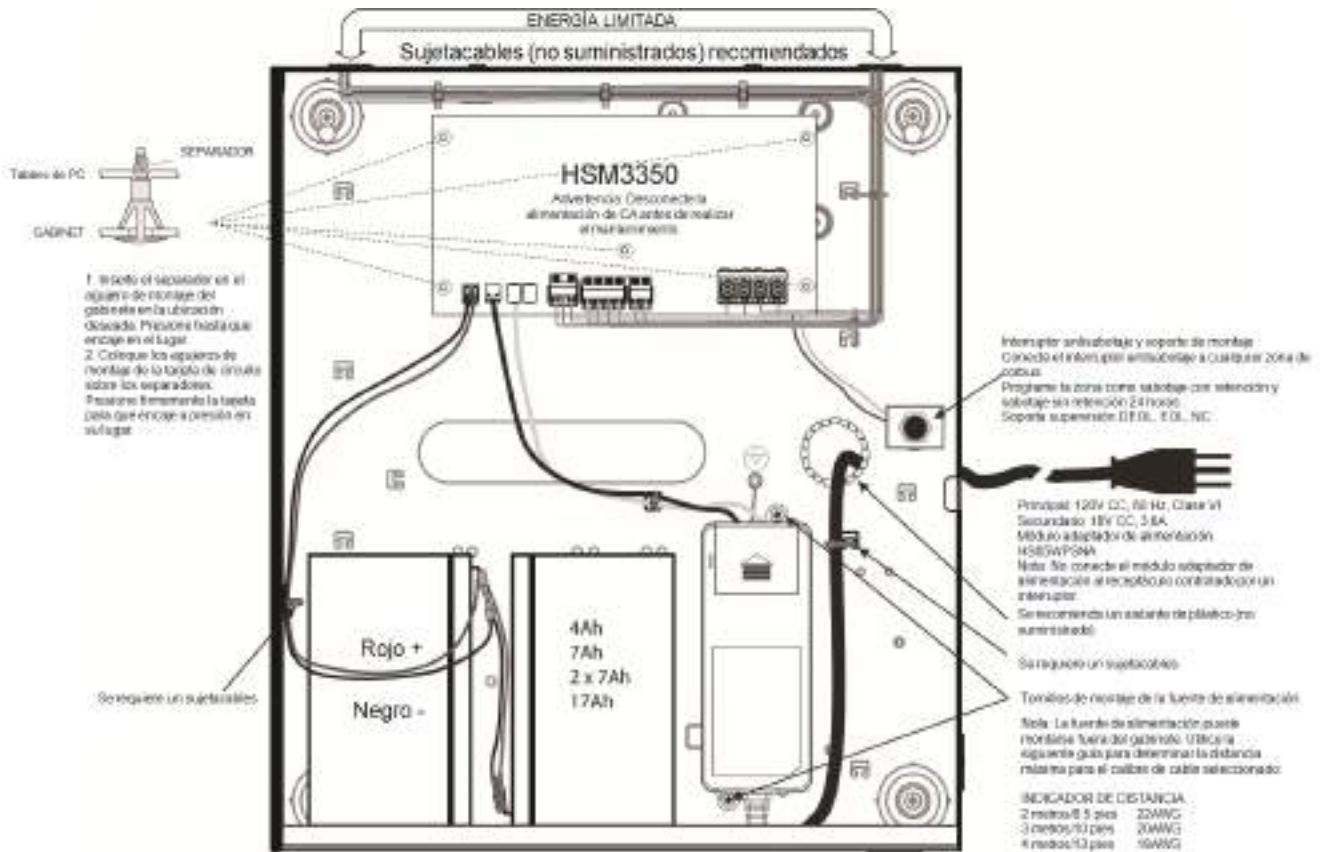
Figure 2-12 HSM3350 en gabinete HSC3010C
