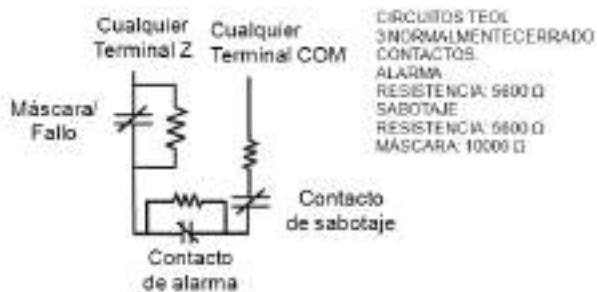
Figure 2-31 TEOL Cableado
