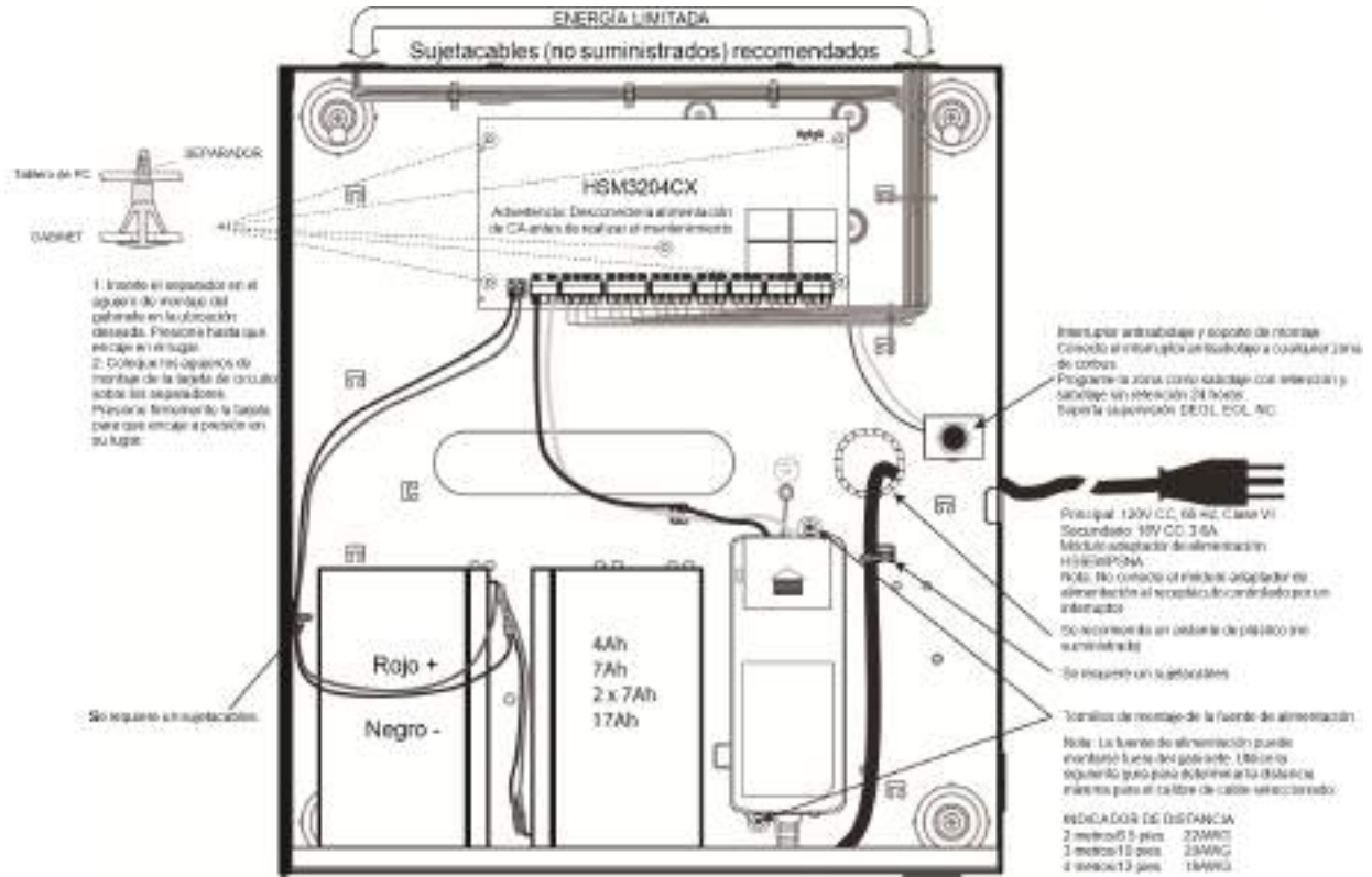
Figure 2-10 HSM3204CX/ HSM3408 en gabinete HSC3010C
