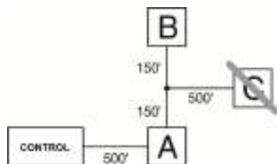
Figure 2-18 Cableado Corbus
