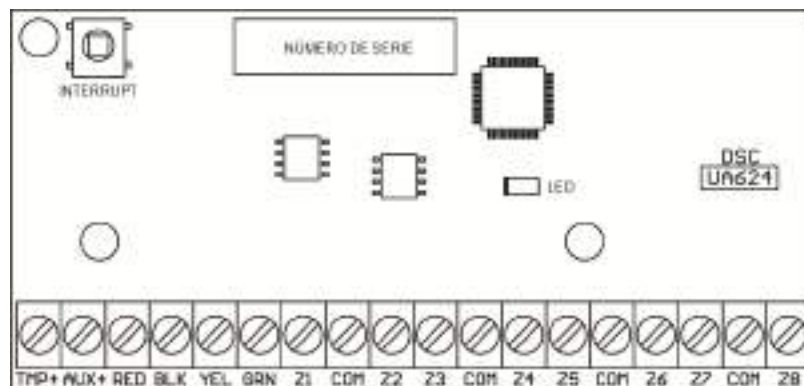
Figure 2-19 Expansor de zona HSM2108
