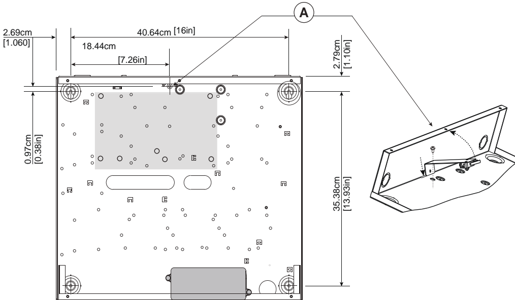
Figure 2-2 Gabinete HSC3020C
