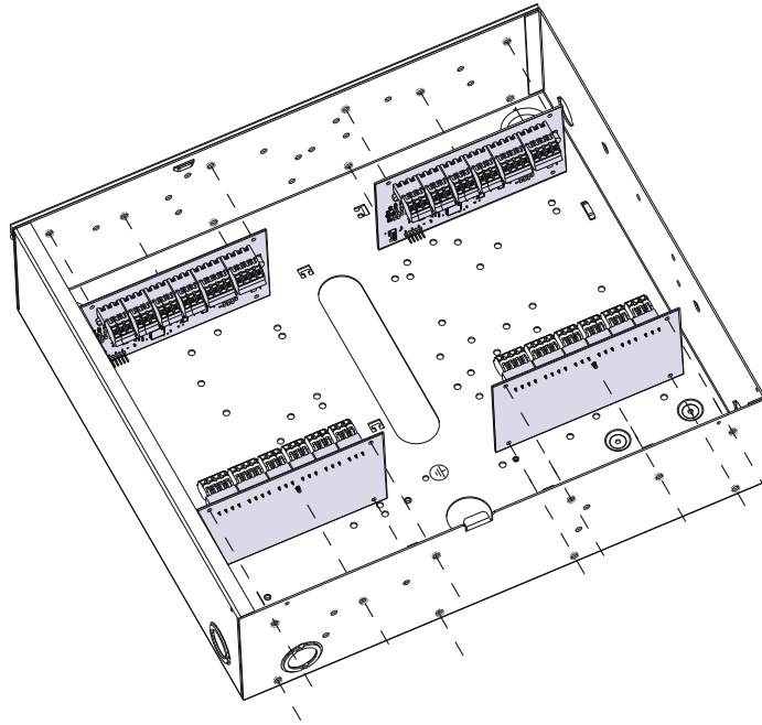
Figure 2-5 HSM3408 en el gabinete HSC3010C
