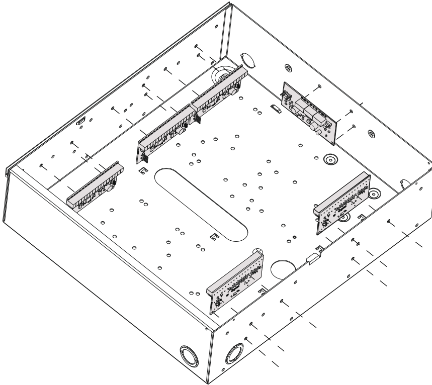
Figure 2-7 Montaje del HSM2108 / HSM2208 en los gabinetes HSC3010C, HSC3010CR, HSC3030CAR
