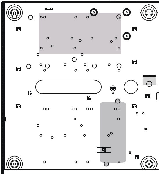
Figure 2-4 Montaje del HSM3304CX/HSM3350 en los gabinetes HSC3010C, HSC3010CR, HSC3030CAR
