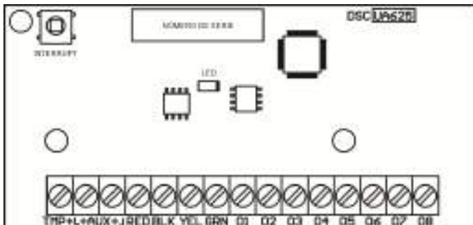
Figure 2-22 HSM2208 Expansor de salida
