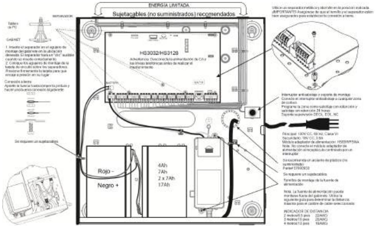
Figure 2-8 Cableado del panel para el HSC3010C
