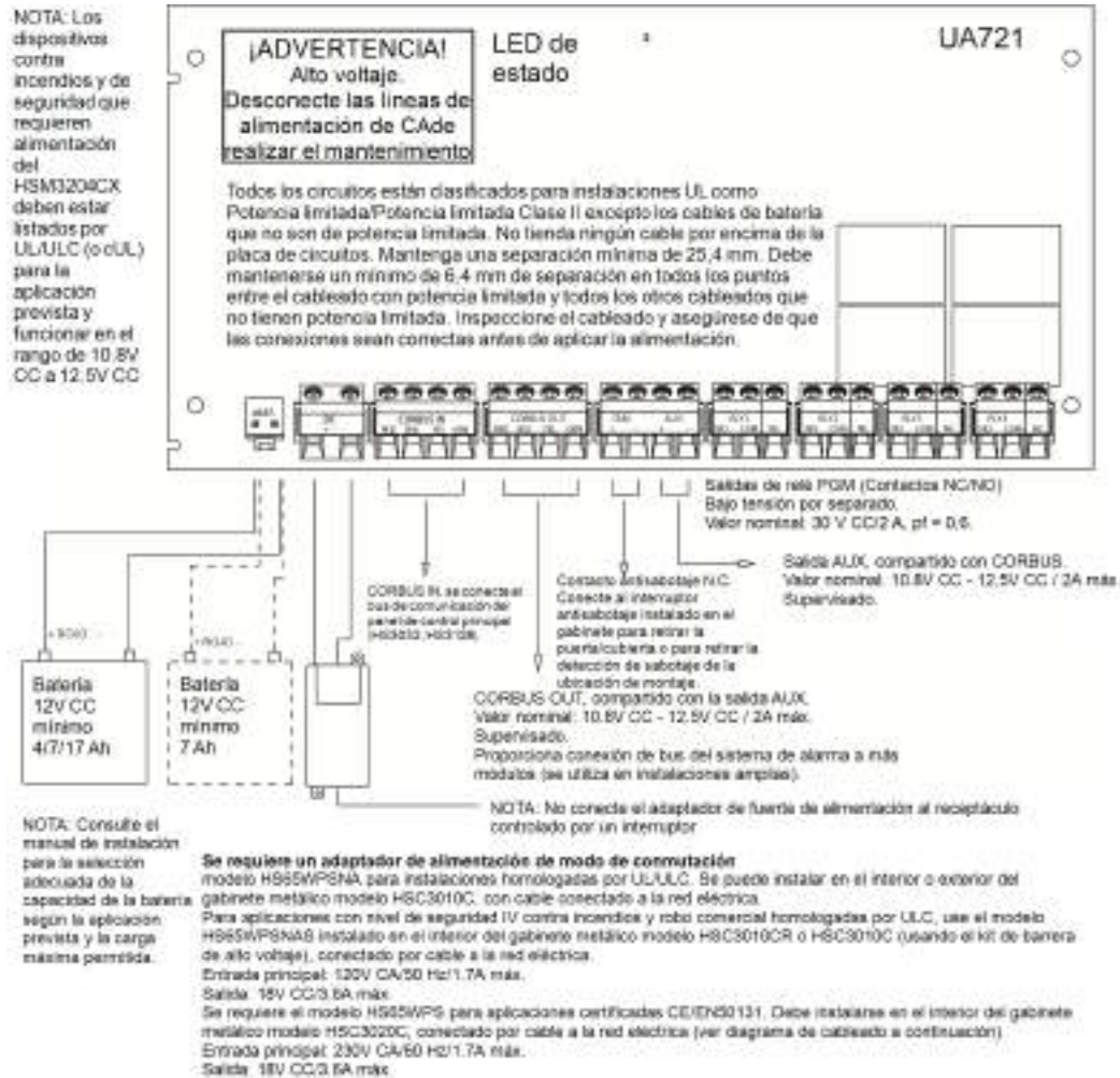
Figure 2-26 Repetidor Corbus HSM3204CX
