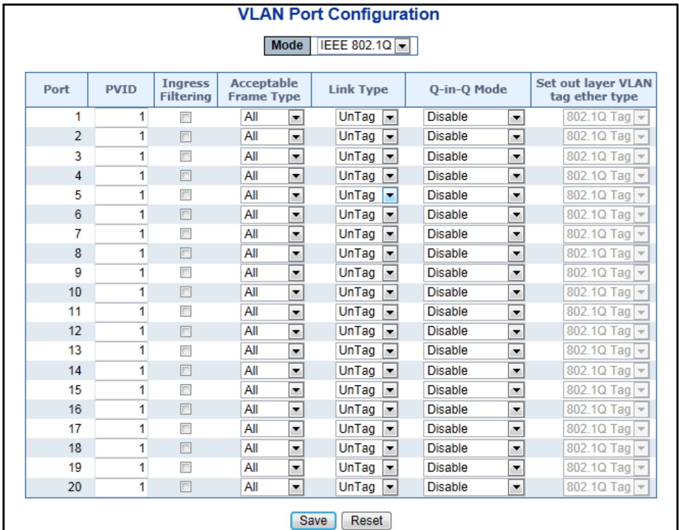
Figure 4-6-2 : VLAN Port Configuration Page Screenshot
