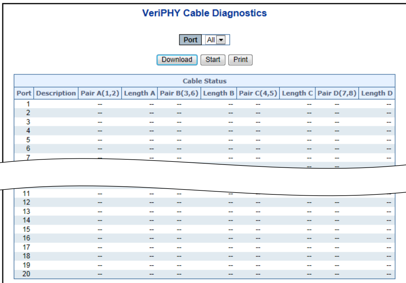
Figure 4-15-4: VeriPHY Cable Diagnostics Page Screenshot
