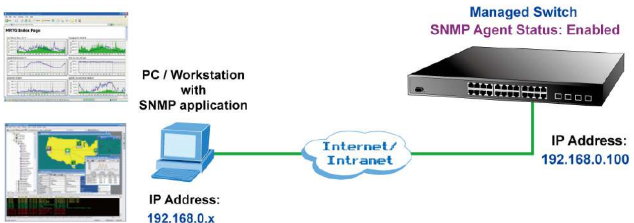
Figure 3-5: SNMP Management
