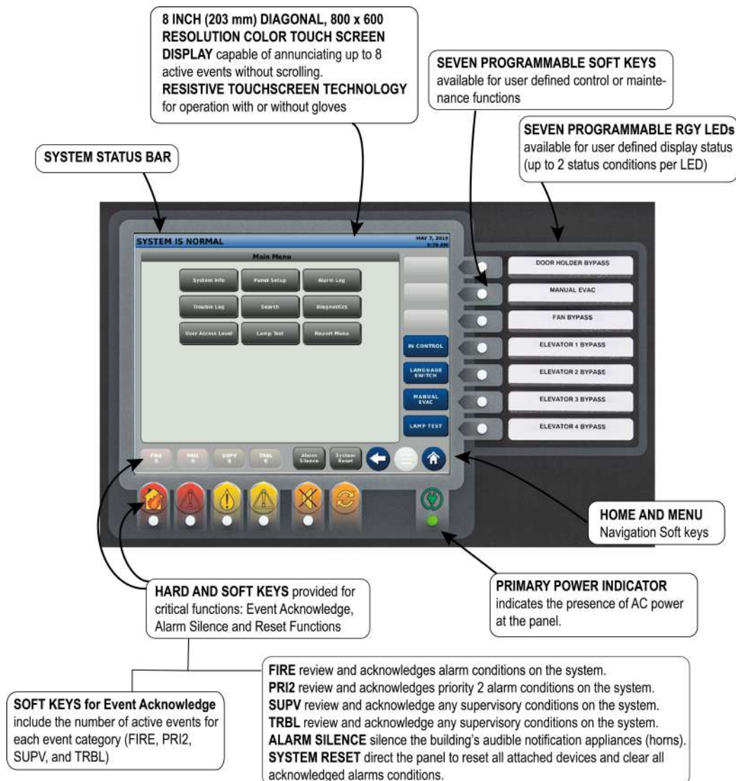
Figure 9: ES Touch Screen Display Operator Interface
