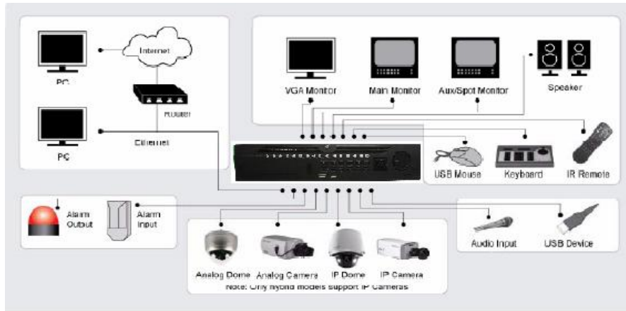
Figure 9 Product Application Diagram
