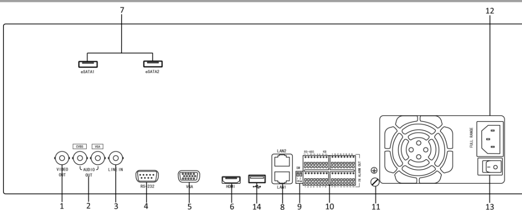
Figure 7 DS-9600NI-XT
