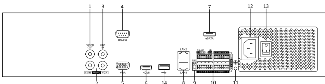
Figure 6 DS-9600NI-ST/RT
