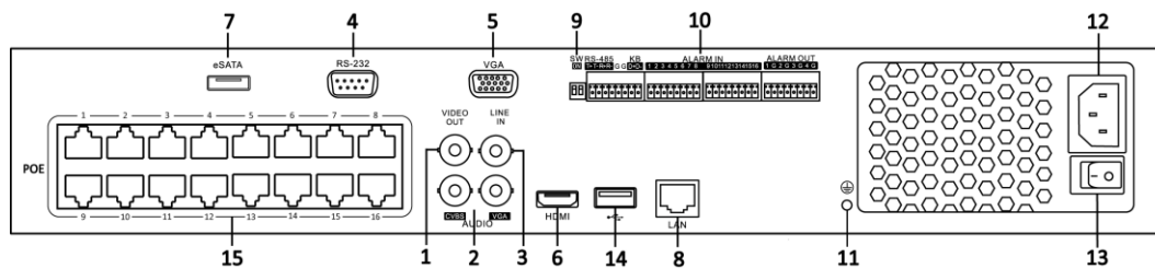
Figure 8 DS-7700NI-SP
