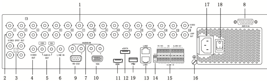
Figure 5 DS-9000HWI-ST & DS-9000HFI-RT
