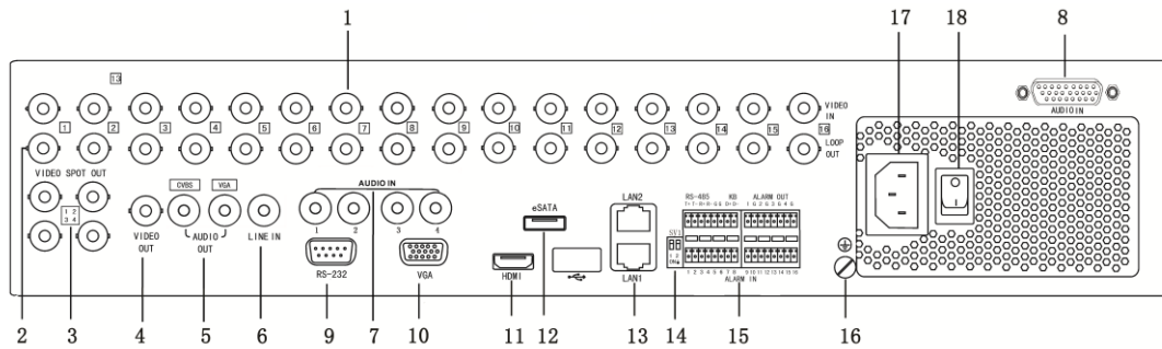
Figure 4 DS-9100/9000HFI-ST
