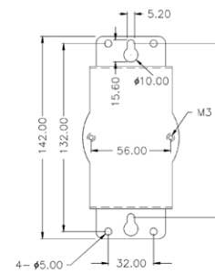
Wall MOUNTING BRACKET
